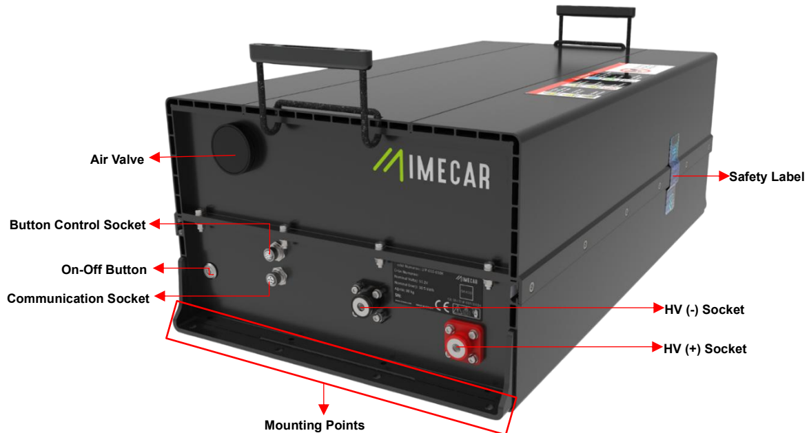
Figure 1 10.5 kWh Battery Pack External View
