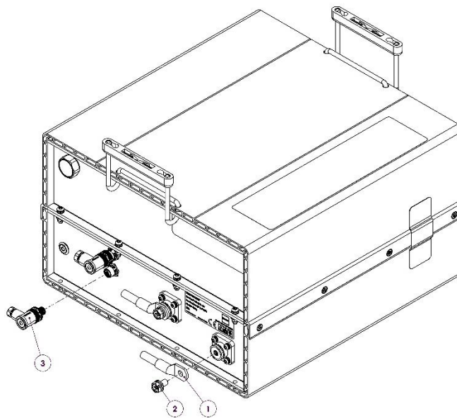
Figure 3 Battery Pack Cable Connection Points
