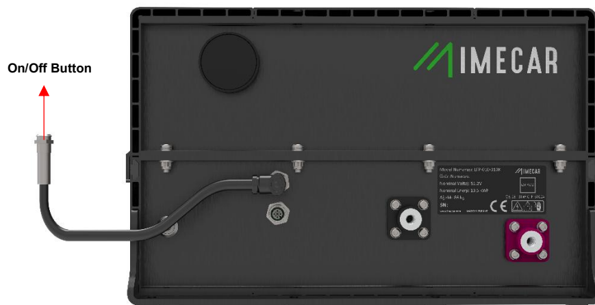
Figure 5 Optional On/Off Button
