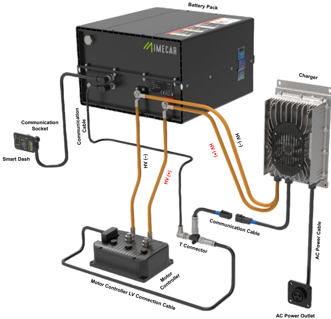
Figure 4 Battery Pack Cable Connections
