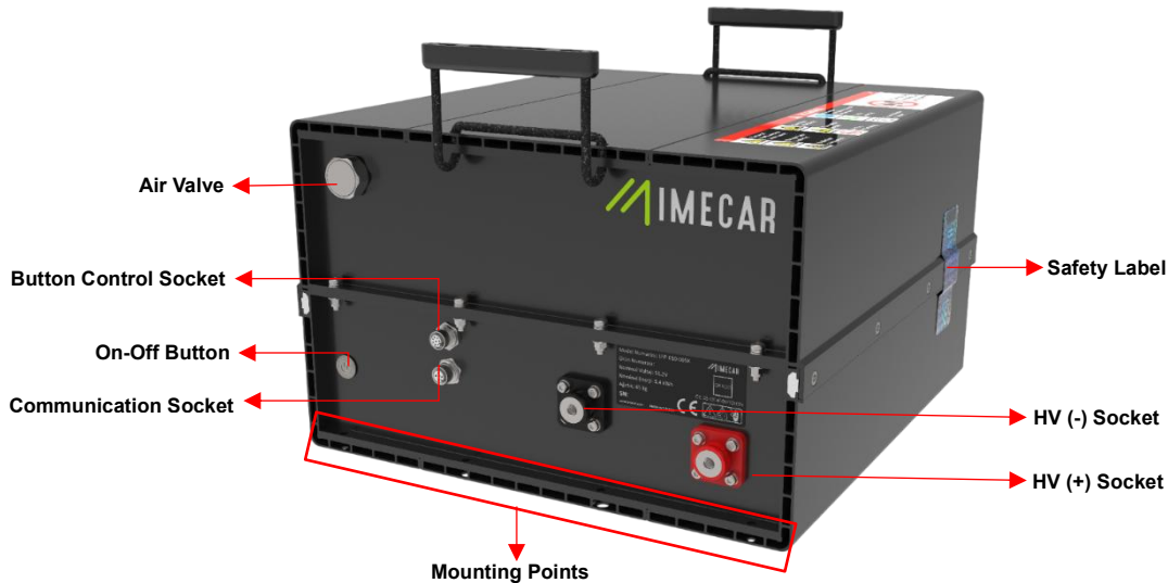
Figure 1 5.4 kWh Battery Pack External View
