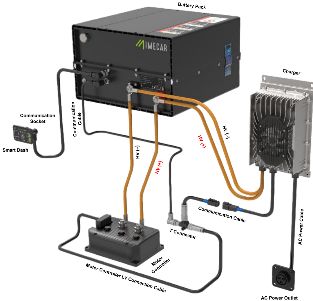
Figure 3 Battery Pack Cable Connections
