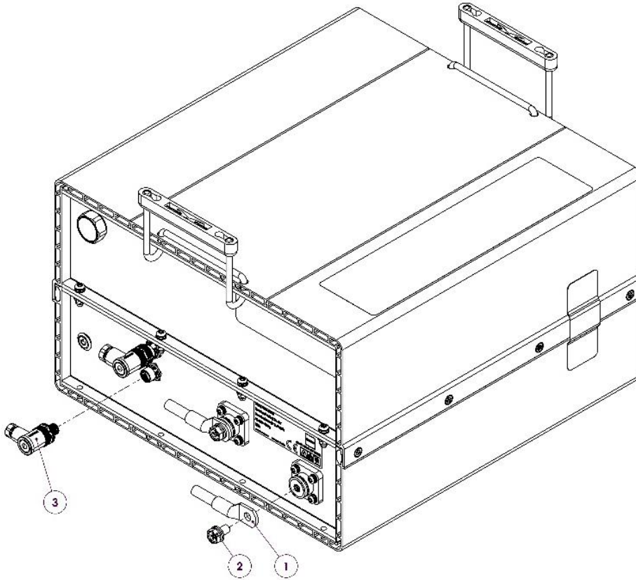
Figure 2 Battery Pack Cable Connection Points
